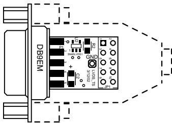
Top Silk Layer + parts layout
